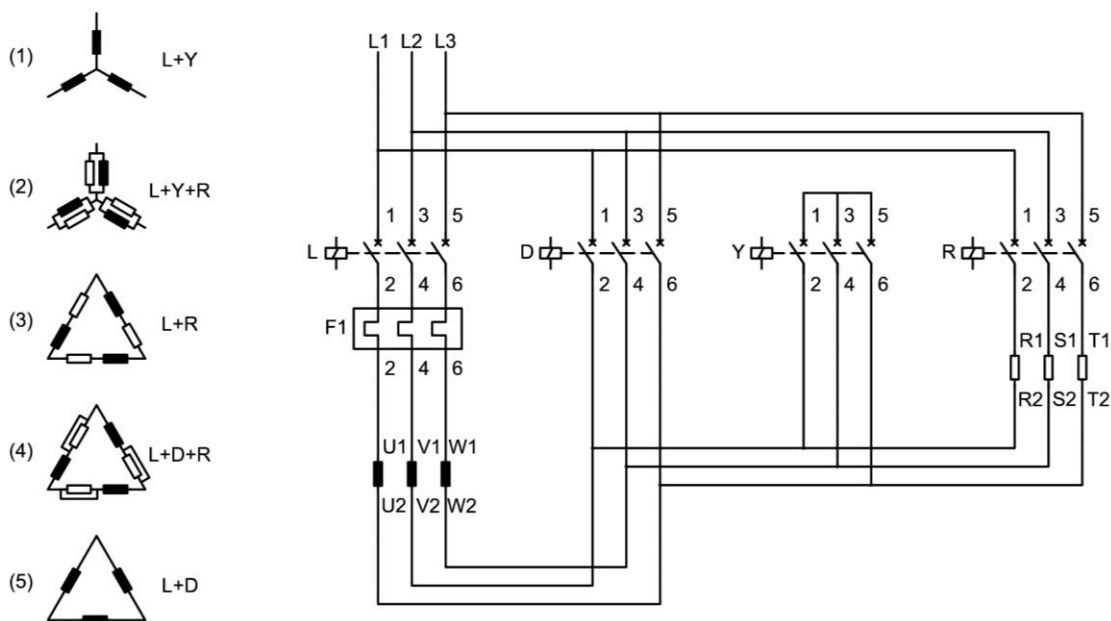
Wiring Diagram for Closed Transition Star-Delta Starter
